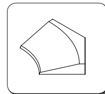
Inside 45 Corner Reducer 12" x 8" x 2-1/2"
