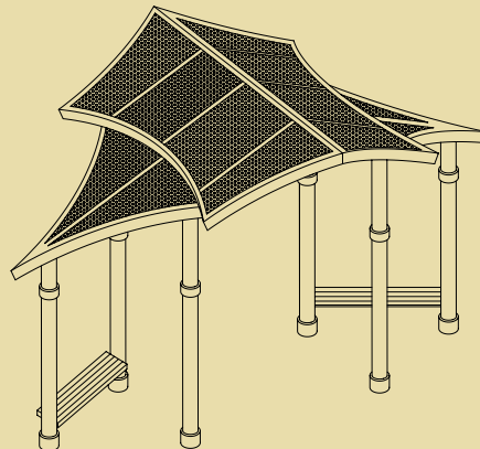
Model 9313-SKD Custom 13'X18' Pittsburgh All-Steel Sky Series Duo-Top Solar shelter featuring Perfa-Lite perforated metal roofing, custom round banded steel columns and straight backless all-steel attached benches
