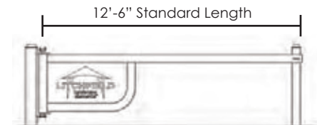
Model CSG-207 Straight Beam Single Swing Gate with laser-cut insert and curved support (we can customize with your logo)
