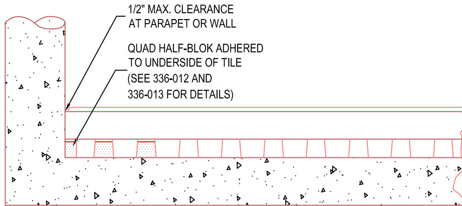
FULL TILE TERMINATION AT PARAPET OR WALL
