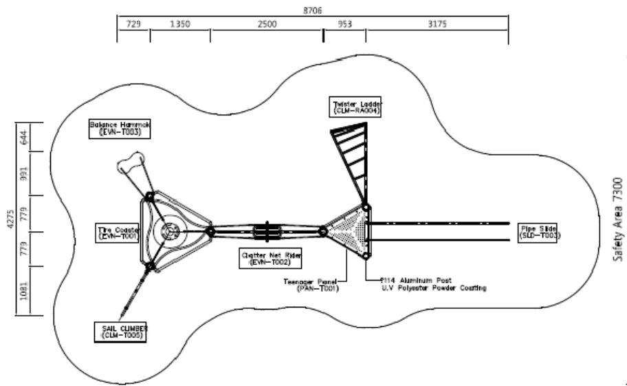
Layout Drawing
