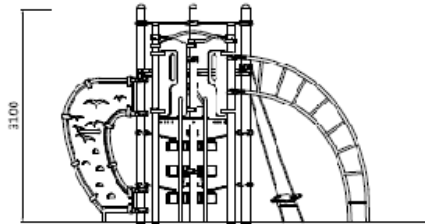
Right View scale : none
