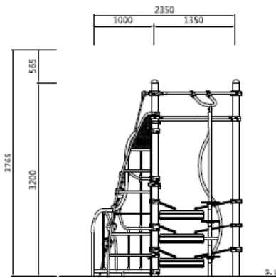
RIGHT DRAWING SCALE: NONE
