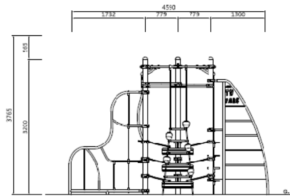
FRONT DRAWING SCALE: 1:100
