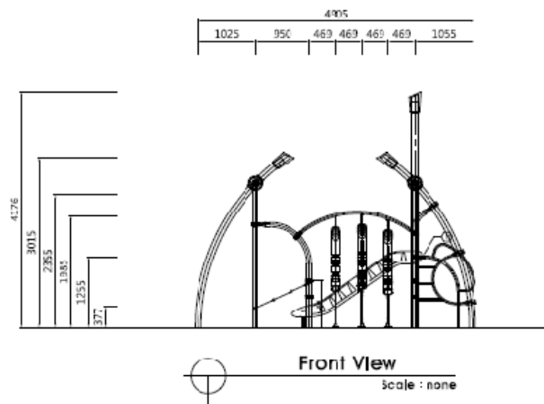
Layout Drawing Scale : none
