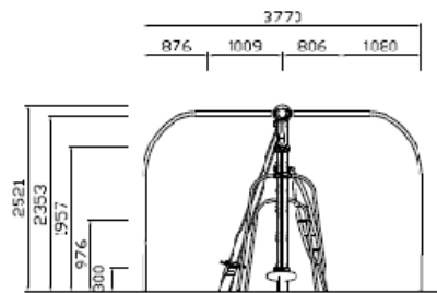
Right View
