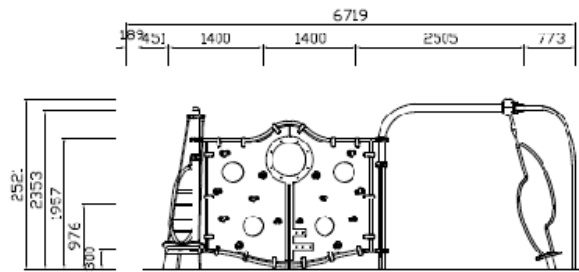
Front View Scale : none
