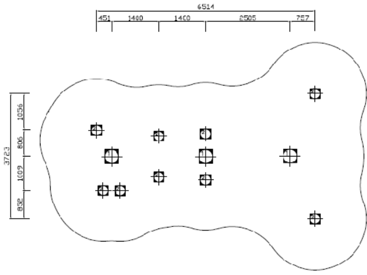
Footing Drawing
