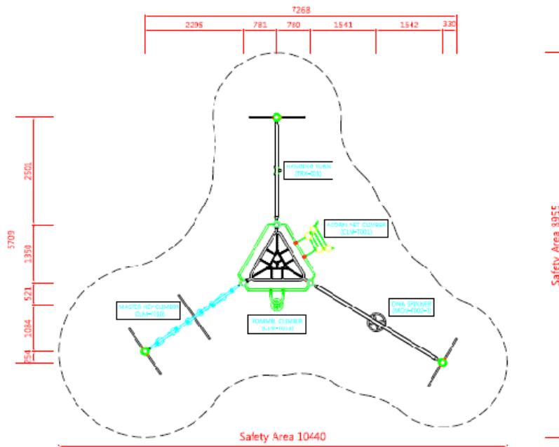
Layout Drawing Scale : none
