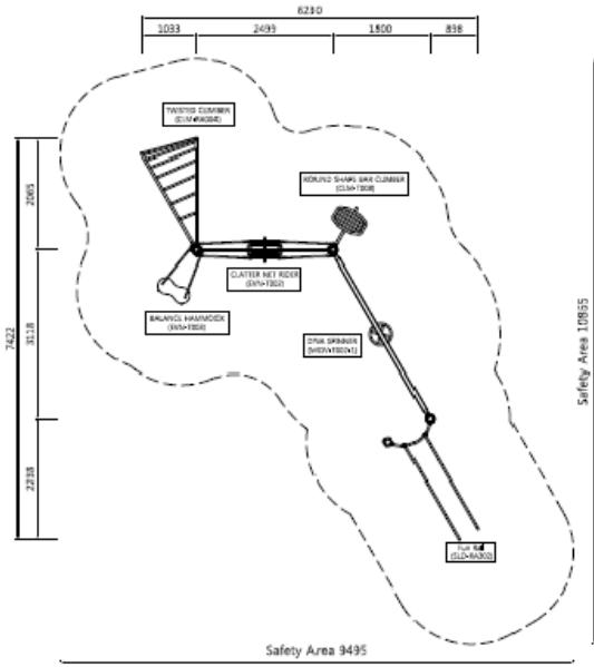
Layout Drawing Scale: none
