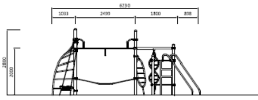
Front View Scale: none
