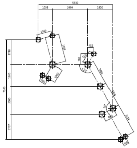
Footings Drawing Scale: none
